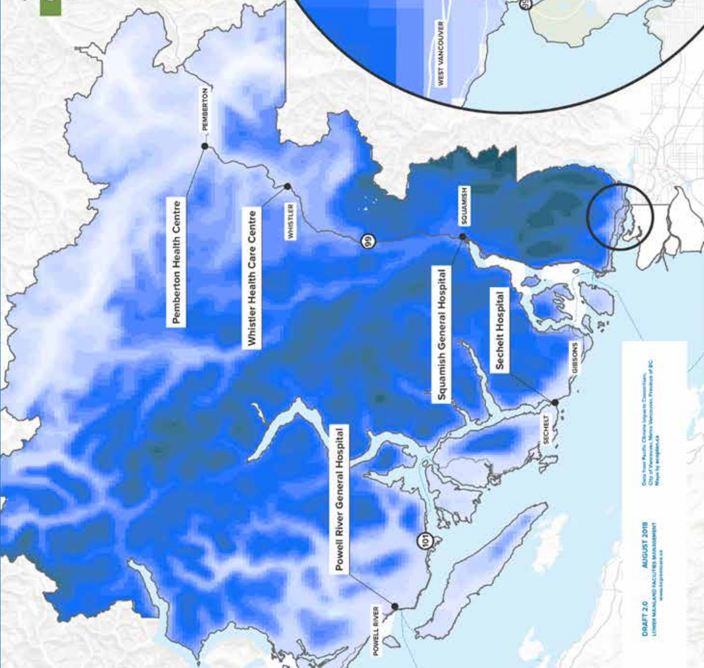
R95P Wettest Day Precipitation - Past
